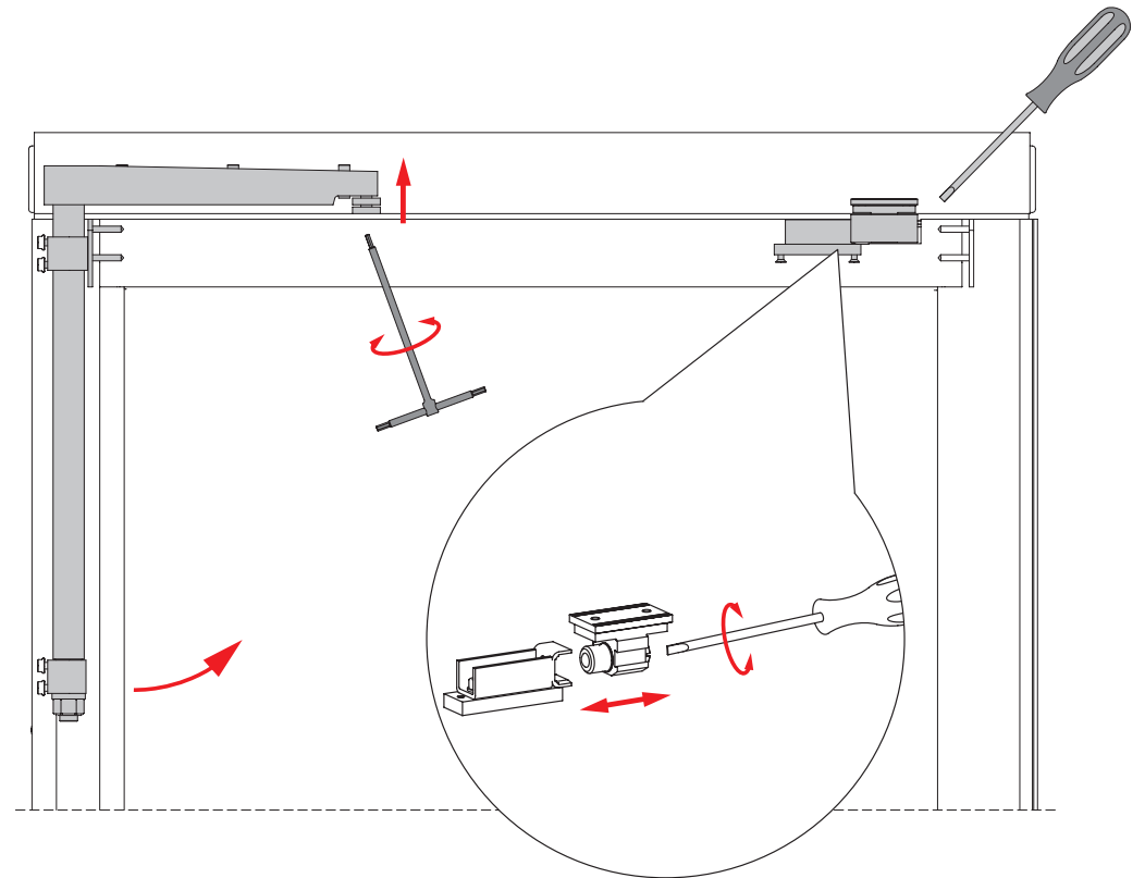
10 Moving door wing regulation
